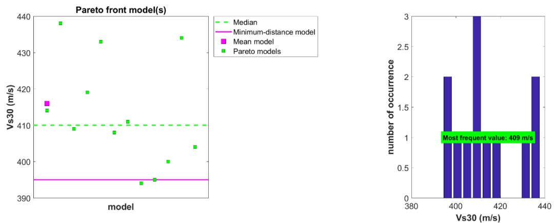
Figura 42. Correlazione Vs30 median, minimum-distance model, mean model, pareto models
